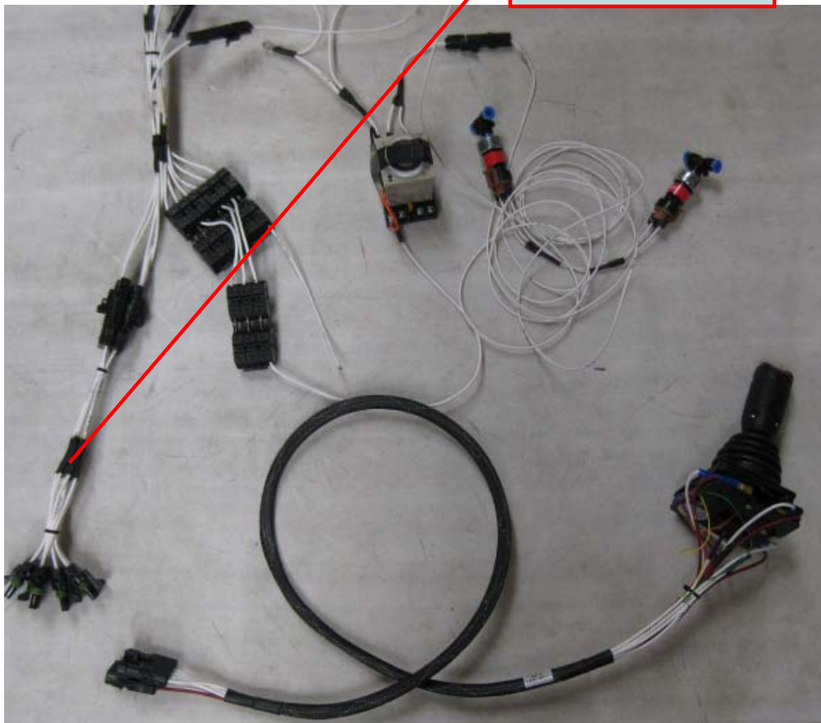
Pigtail Splitter
